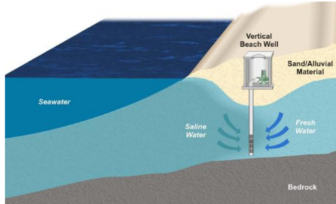
Figure B-1 Vertical Wells
