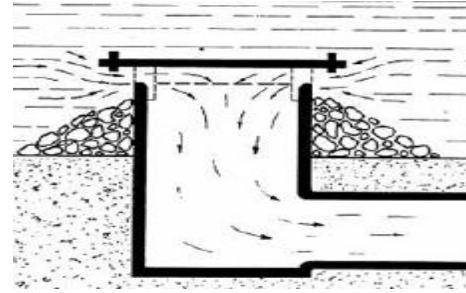
Figure B-3 Velocity Cap Illustration
