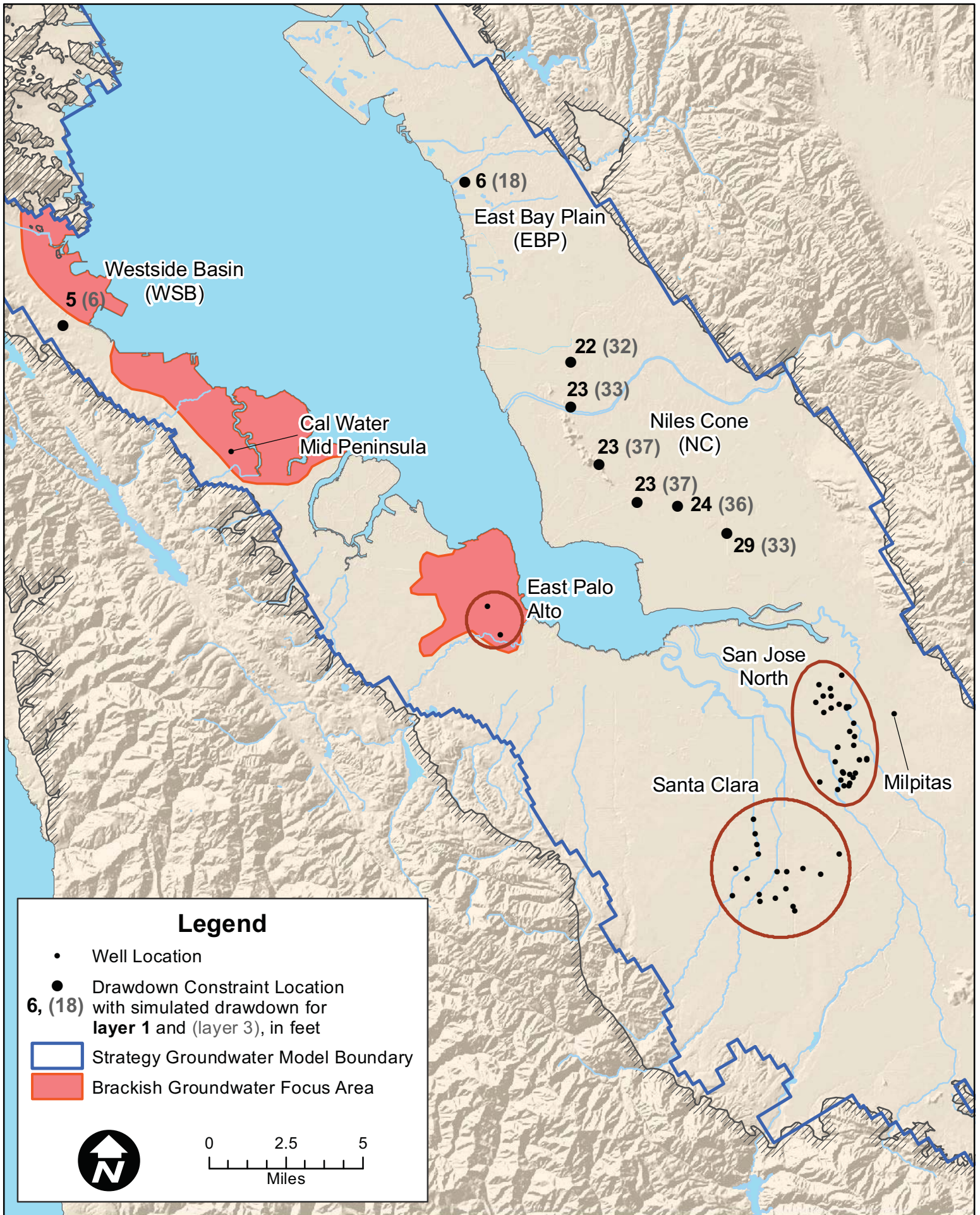
Figure 01H Simulated Regional Drawdown Effect for Future Increases in BAWSCA Agency Groundwater Use
